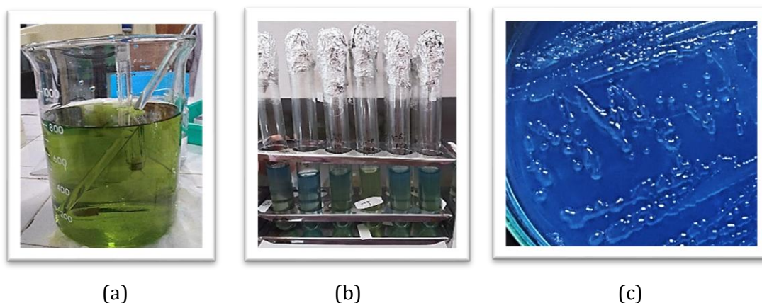
Figure 3. (a) The production of Nitrogen-Free Bacteria (NFB) media; (b) Isolation of Nitrogen-Fixing Bacteria on NFB media (broth); (c) Colonies of Nitrogen-Fixing Bacteria on NFB media.
