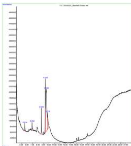
Figure 5. Gas separation chromatogram graph of purple phenotype flower of-Kesiman Kertalangu.
