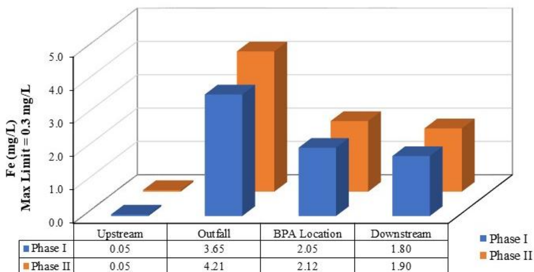
Figure 10. Iron standard quality comparison with the water quality standard
