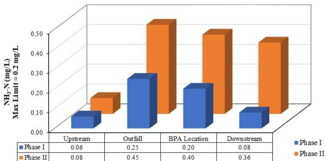
Figure 9. \text{NH}_3\text{-N} standard quality comparison with the water quality standard
